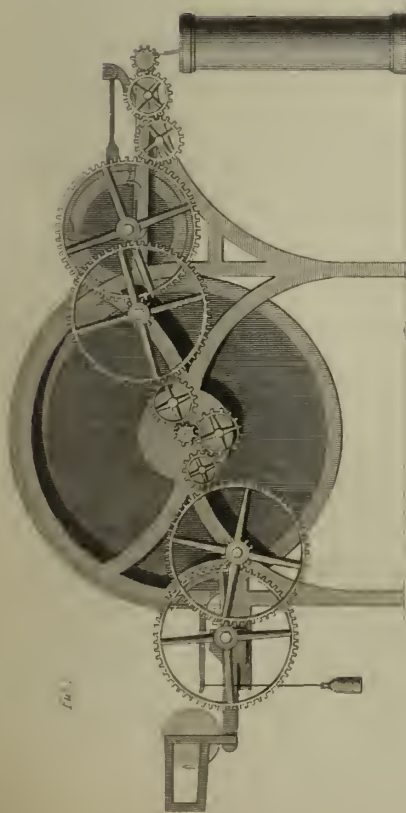
Carding Engine End Elevation
