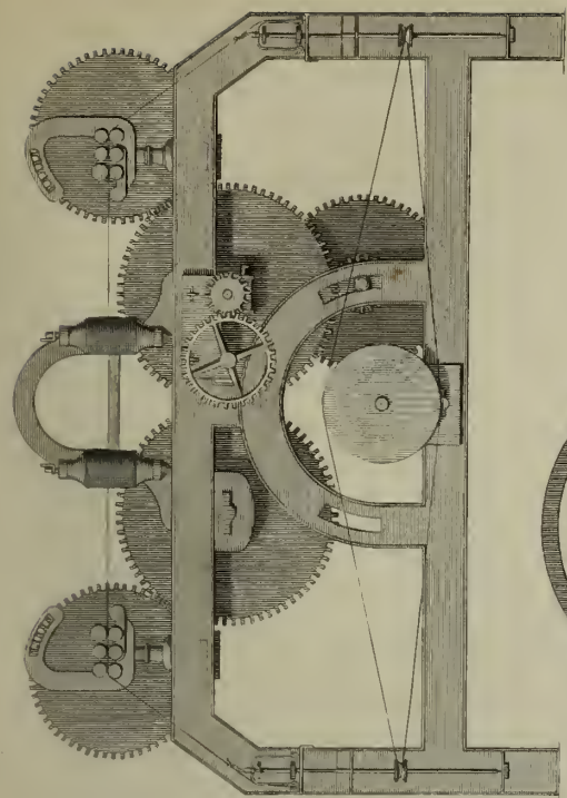
Throstle End Elevation
